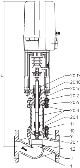
Fig. 441 Bellows seal
